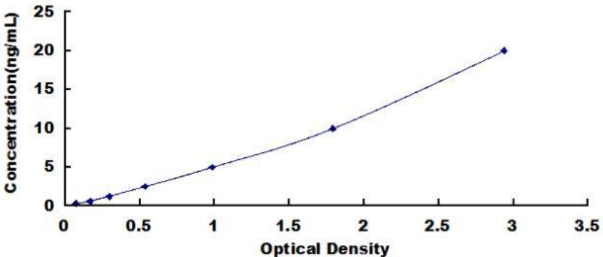
Typical Standard Curve for Human TAF A2 ELISA.
