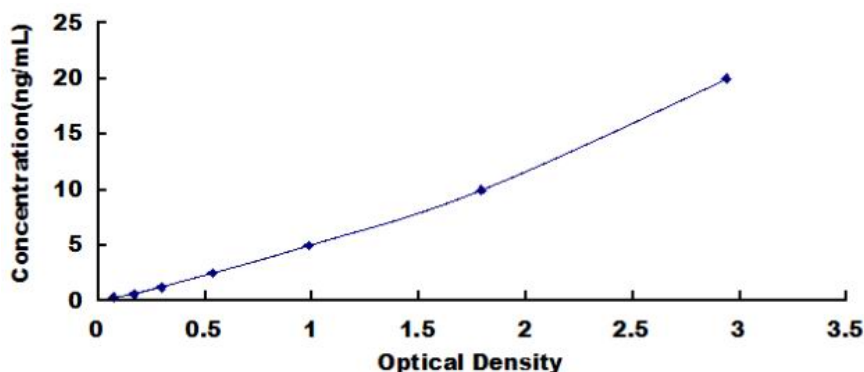
Typical Standard Curve for Human SHC1 ELISA.
