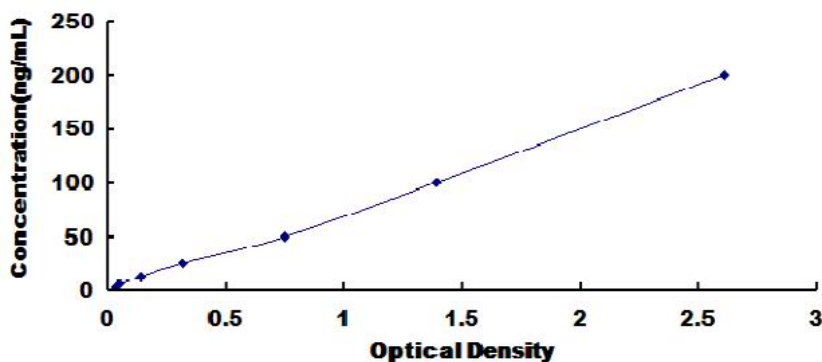
Typical Standard Curve for Rat PCSK1 ELISA.
