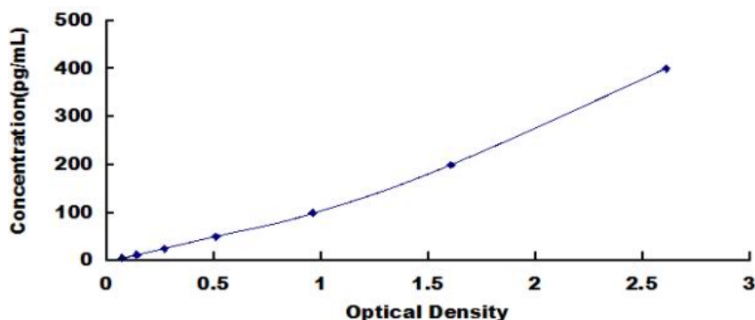
Typical Standard Curve for Rat MIP3a ELISA.
