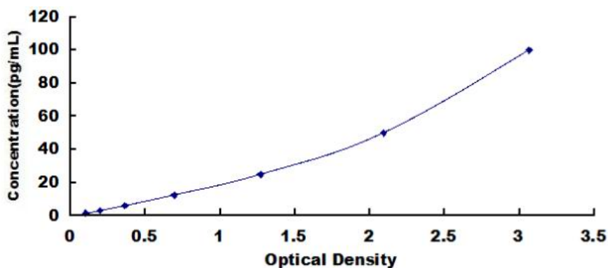
Typical Standard Curve for Rat MIF ELISA.
