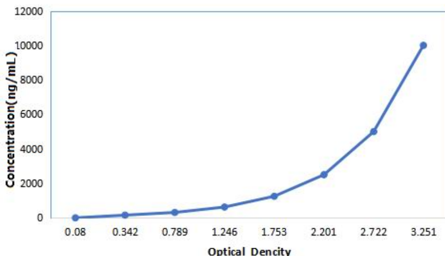
Typical Standard Curve for Rat LDL ELISA.
