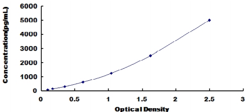
Typical Standard Curve for Porcine INS ELISA.
