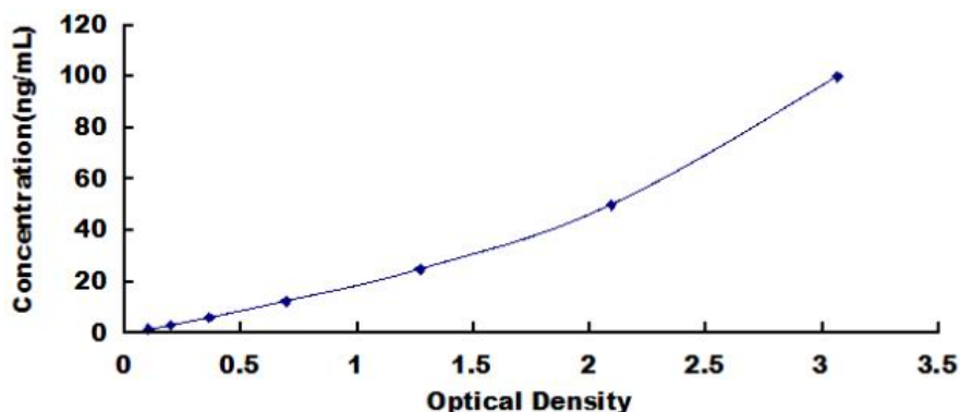
Typical Standard Curve for Human INHBP ELISA.
