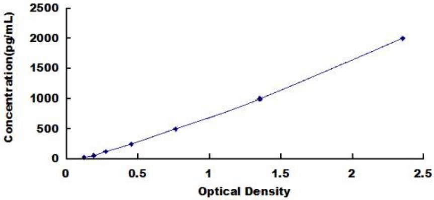
Typical Standard Curve for Human IK ELISA.
