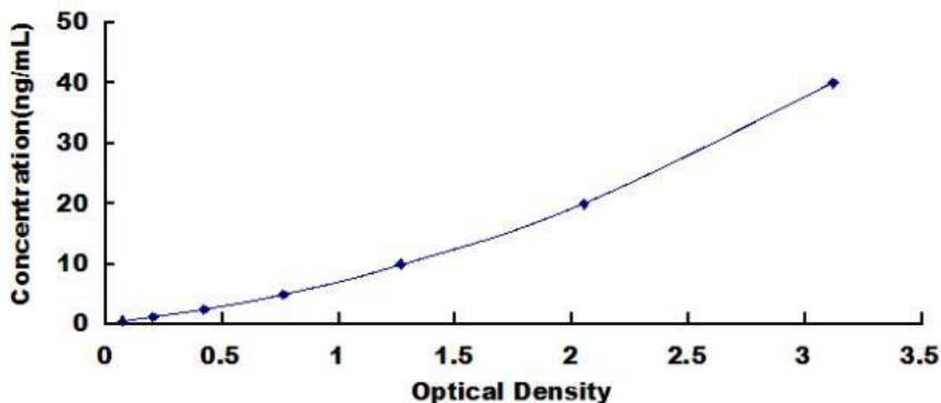
Typical Standard Curve for Rat IGFBP3 ELISA.
