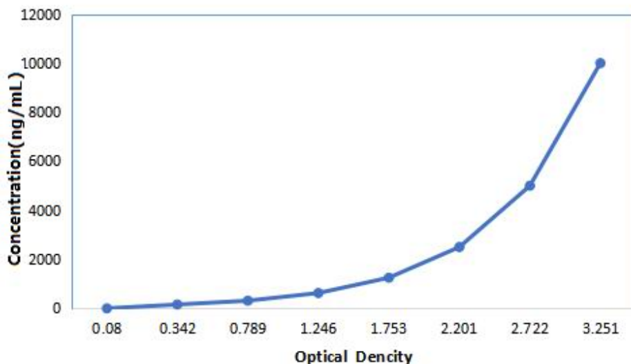
Typical Standard Curve for Bovine Hpt ELISA.
