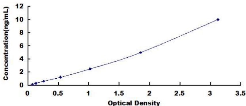
Typical Standard Curve for Human HSPA1A ELISA.
