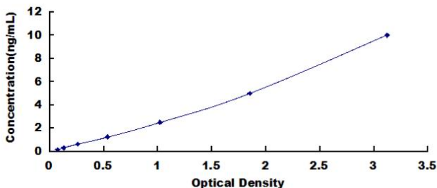
Typical Standard Curve for Human HEMGN ELISA.
