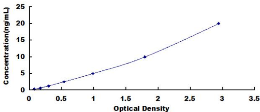
Typical Standard Curve for Mouse GLUT3 ELISA.
