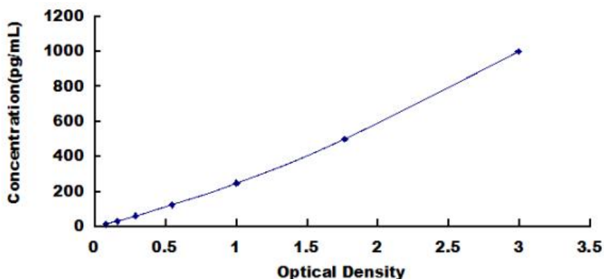
Typical Standard Curve for Mouse GHRH ELISA.
