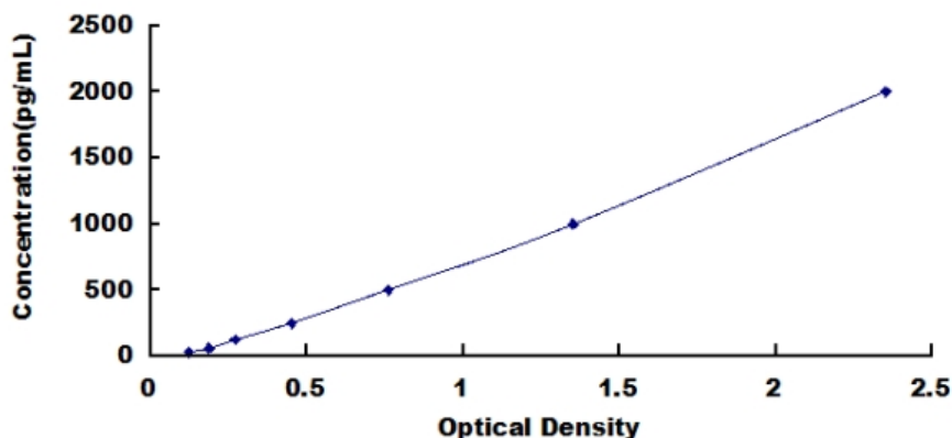
Typical Standard Curve for Mouse GFAP ELISA.
