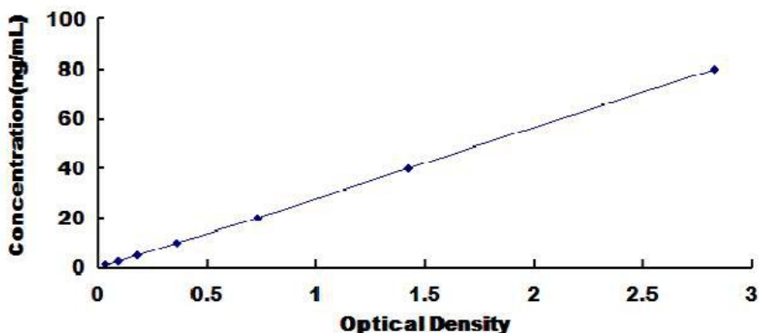
Typical Standard Curve for Human FcgR3B ELISA.
