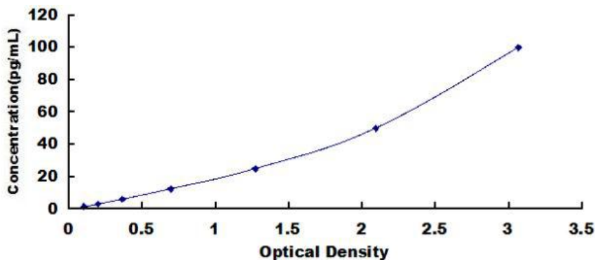
Typical Standard Curve for Mouse FcεRII ELISA.
