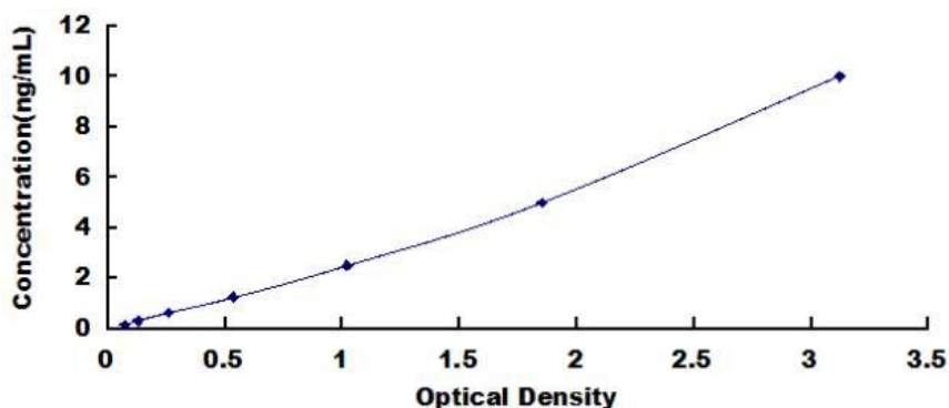
Typical Standard Curve for Human DCTD ELISA.
