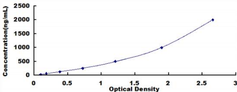
Typical Standard Curve for Bovine CSN1 ELISA.
