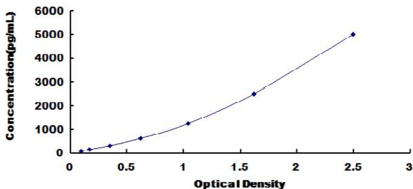
Typical Standard Curve for Mouse ALPK3 ELISA.
