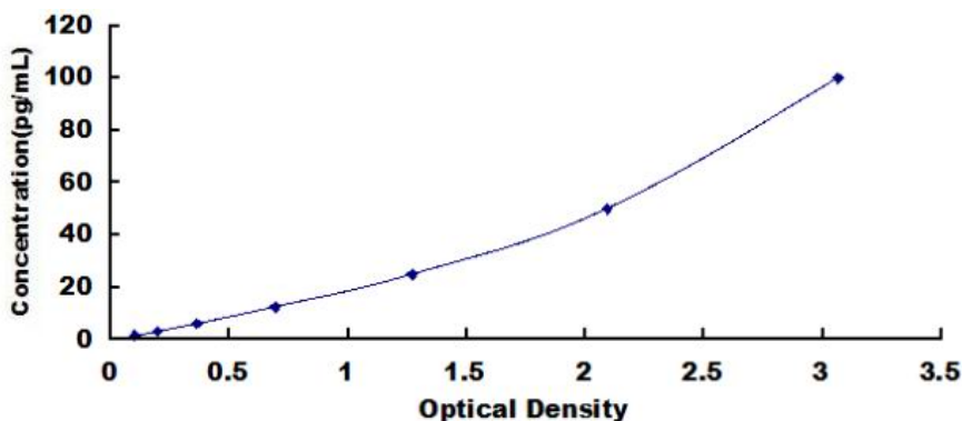
Typical Standard Curve for Human TAT ELISA.
