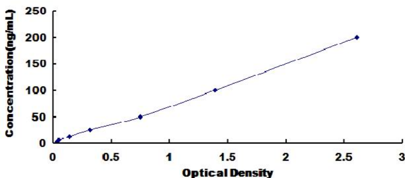
Typical Standard Curve for Rabbit IgM ELISA.
