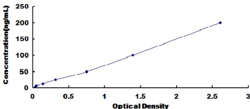
Typical Standard Curve for Mouse IgM ELISA.
