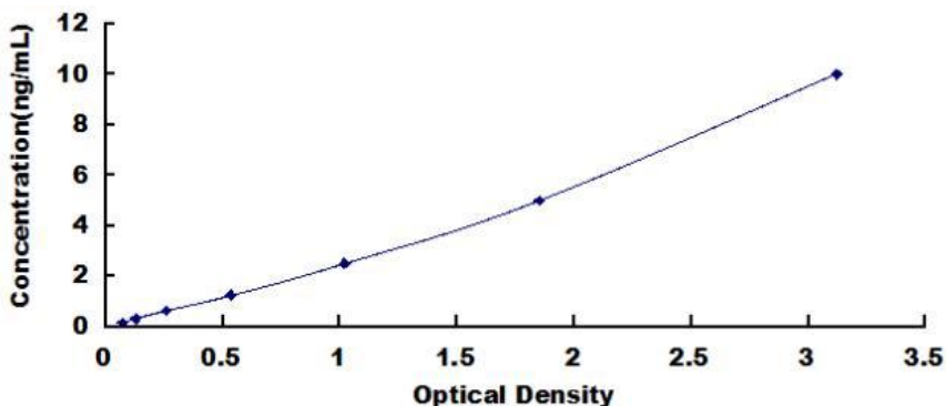
Typical Standard Curve for Rat HSPA1A ELISA.
