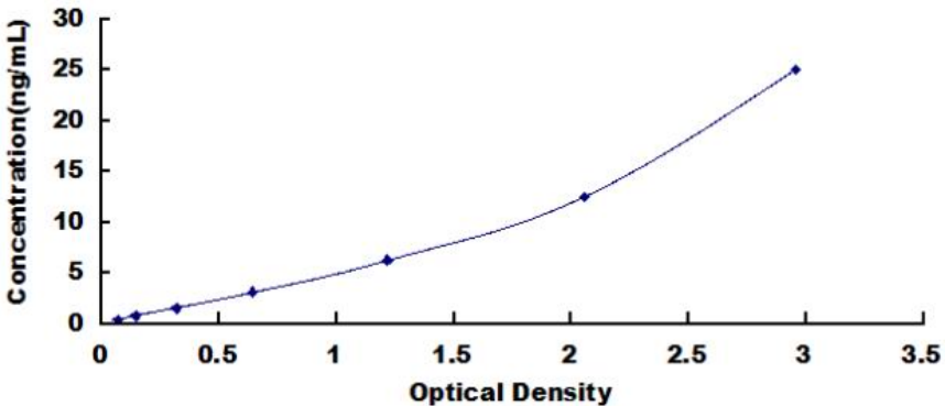
Typical Standard Curve for Mouse VCAM1 ELISA.
