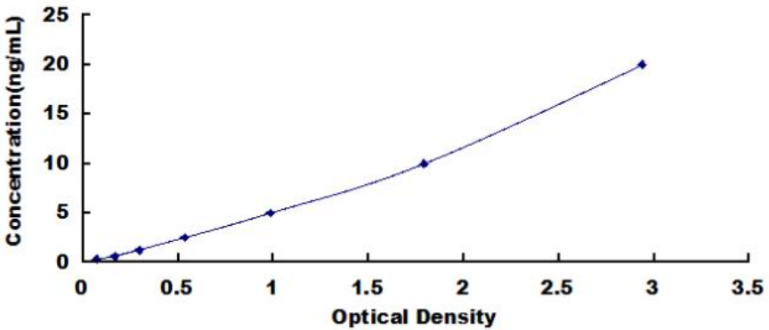
Typical Standard Curve for Human SPINK5 ELISA.
