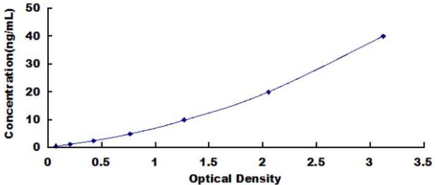
Typical Standard Curve for Porcine SELE ELISA.
