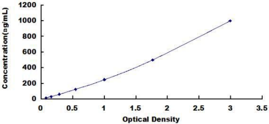
Typical Standard Curve for Equine RNASE5 ELISA.
