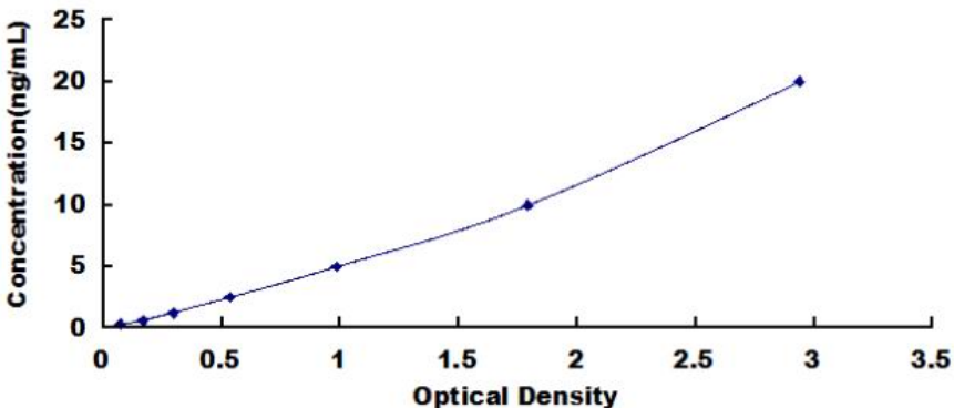
Typical Standard Curve for Human RCN2 ELISA.
