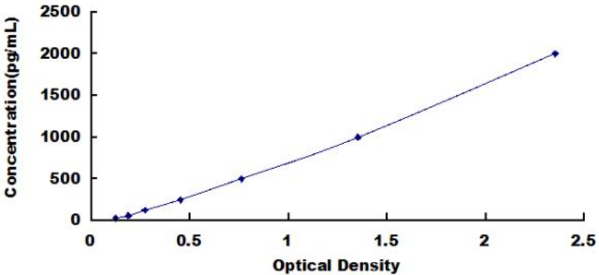
Typical Standard Curve for Human PRDX4 ELISA.
