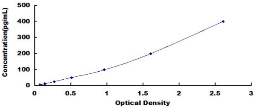
Typical Standard Curve for Human PLA2G2A ELISA.
