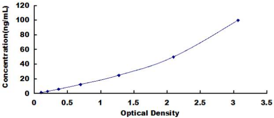
Typical Standard Curve for Mouse ChAT ELISA.
