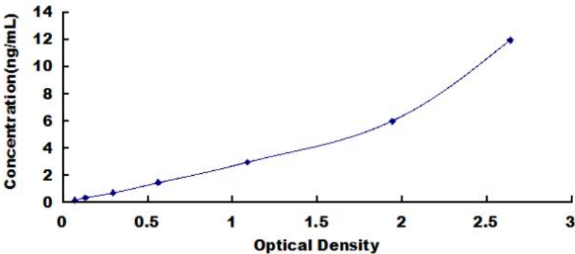
Typical Standard Curve for Human CLEC3B ELISA.
