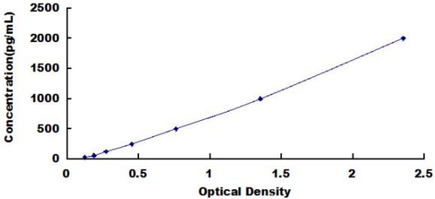
Typical Standard Curve for Human CER ELISA.
