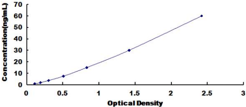
Typical Standard Curve for Bovine CDHE ELISA.
