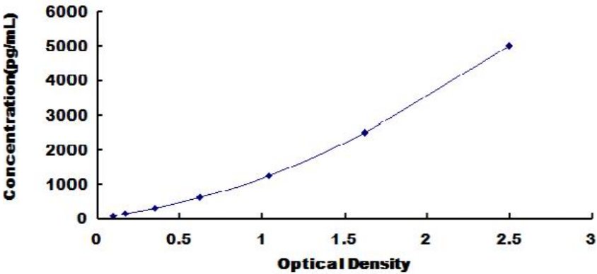
Typical Standard Curve for Mouse CD83 ELISA.
