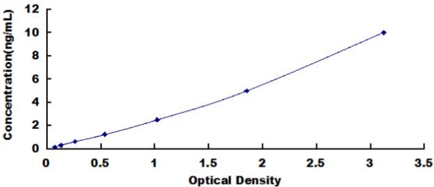
Typical Standard Curve for Chicken CAV1 ELISA.
