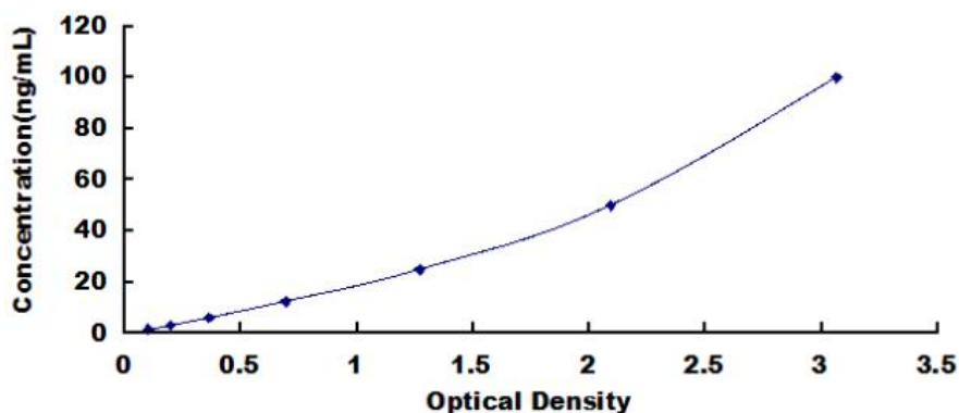
Typical Standard Curve for Rat CAT ELISA.
