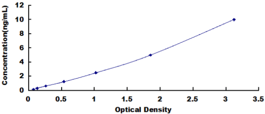
Typical Standard Curve for Human CASP2 ELISA.
