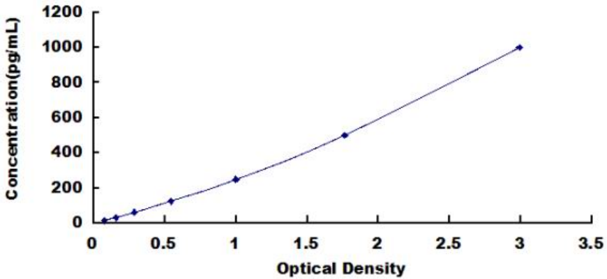
Typical Standard Curve for Rat CART ELISA.
