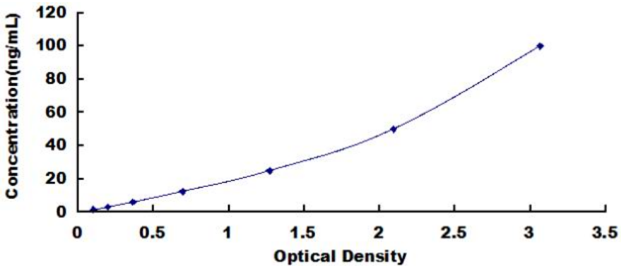
Typical Standard Curve for Human CAP3 ELISA.
