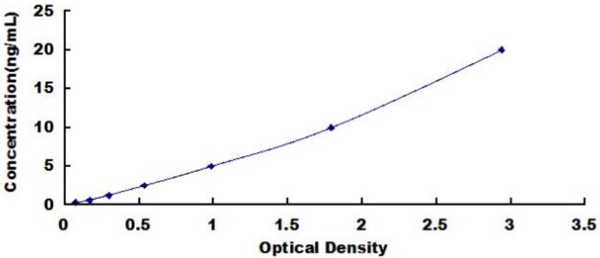
Typical Standard Curve for Human CA72-4 ELISA.
