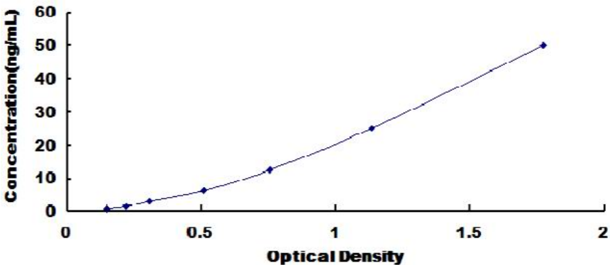
Typical Standard Curve for Human C1qR1 ELISA.
