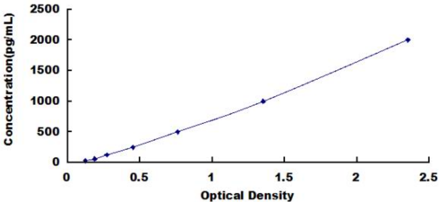
Typical Standard Curve for Mouse BNP ELISA.
