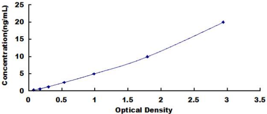
Typical Standard Curve for Rat BECN1 ELISA.
