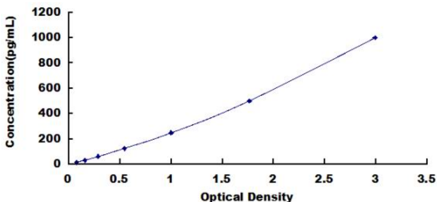
Typical Standard Curve for Mouse AREG ELISA.
