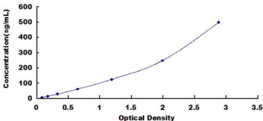
Typical Standard Curve for Mouse APOC2 ELISA.
