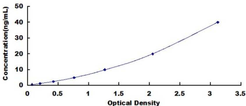
Typical Standard Curve for Bovine ANXA5 ELISA.
