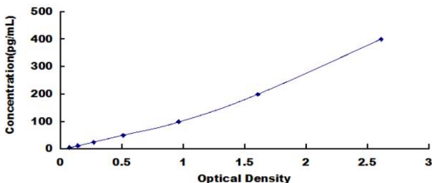
Typical Standard Curve for Mouse ANGPTL2 ELISA.
